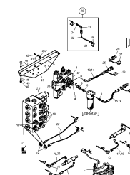
ETB-000943, Hydraulika Comfort
